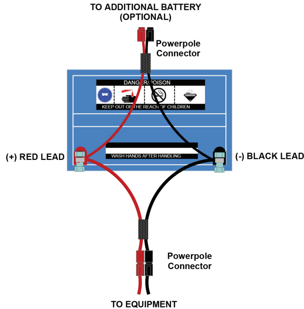
Figure 1: +12 Volt Single SLA Battery Configuration
